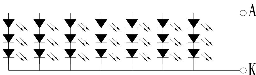
Backlight LED Circuit V_F=9.6\text{V(TYP)} , I_F=140\text{mA}
