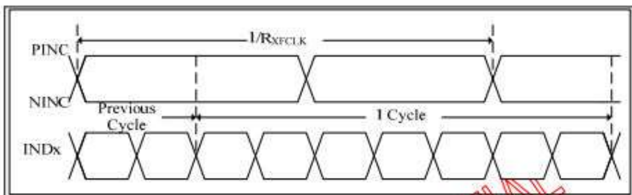
LVDS timing(1)
