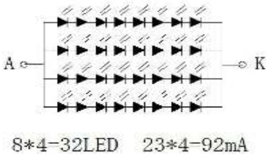
LED Circuit Diagram
