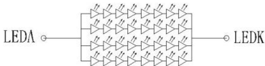
Backlight LED Circuit 8串4并32LED, 80mA /25.6V)
