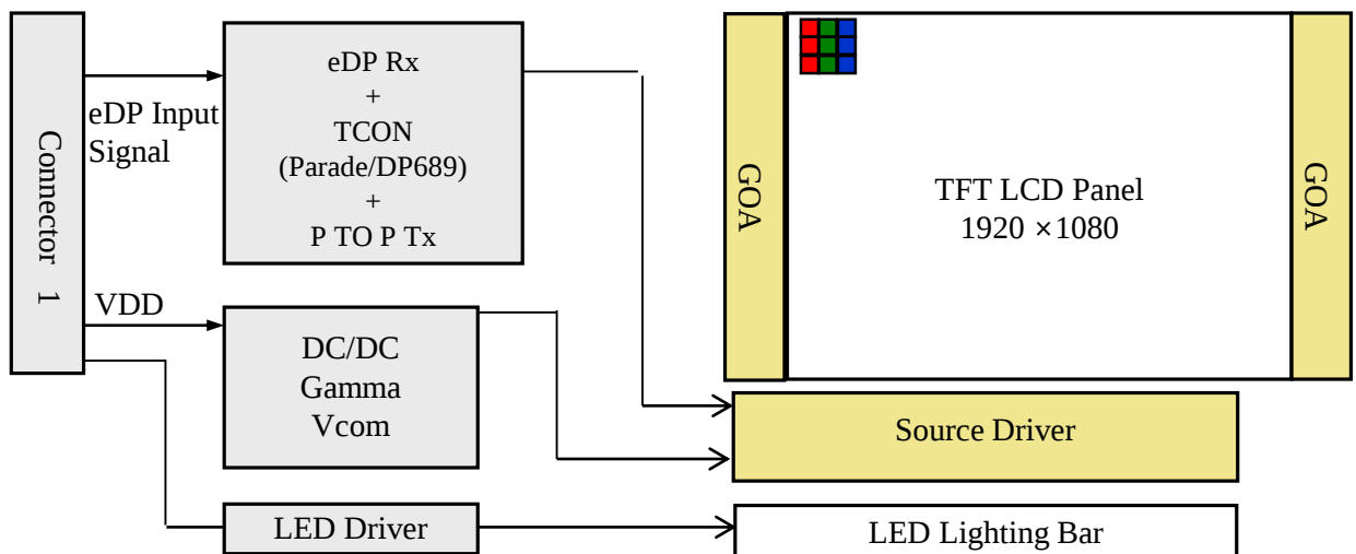
Figure 1. Drive Architecture
