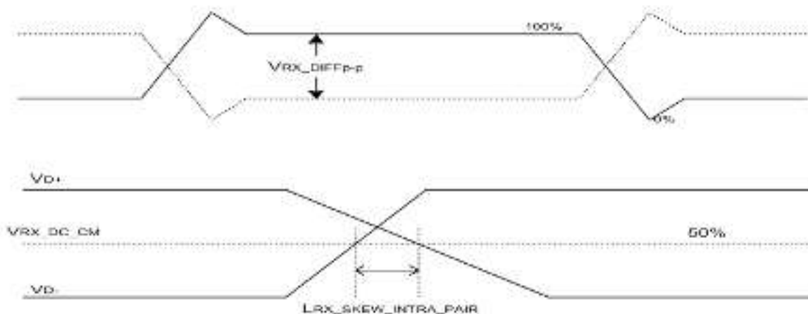
Figure 14. VRX-DIFFp-p & LRX_SKEW_INTRA_PAIR
