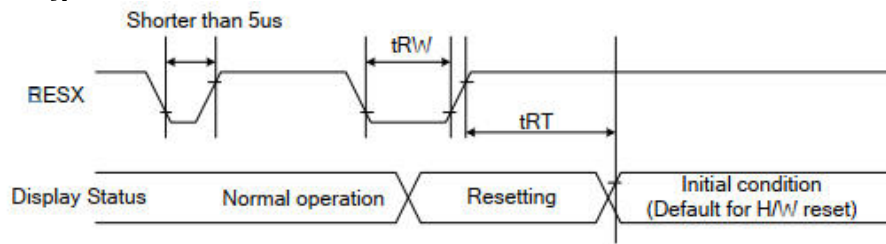
Figure 113: Reset Timing
