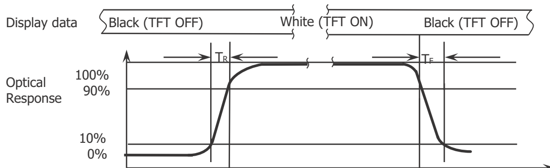
Figure 3. Response Time Testing
