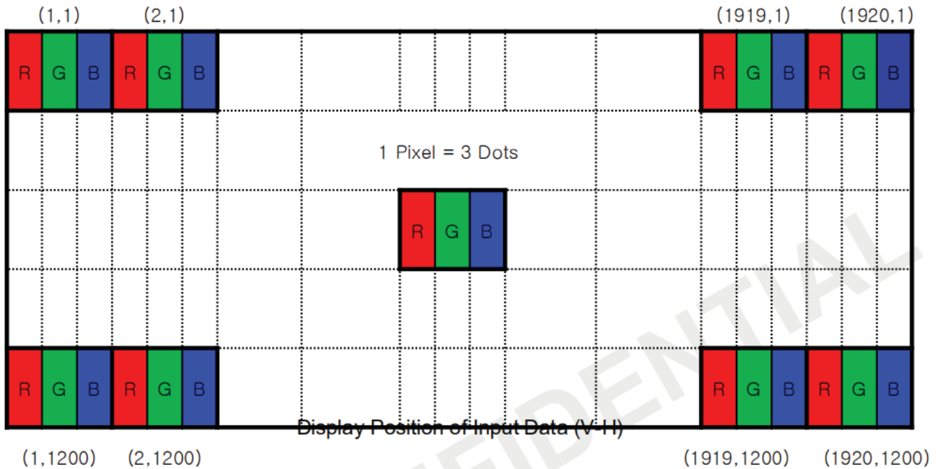
Figure 5. Pixel Format
