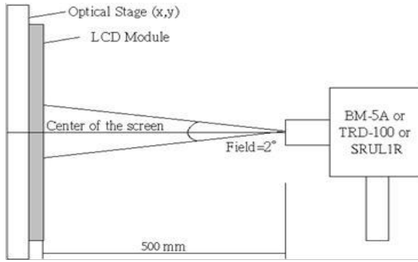
Figure 2. Response Time Testing
