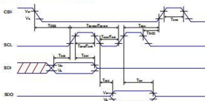
Figure: 3-pin Serial Interface Characteristics
